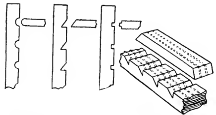
FIG. 456. ADJUSTABLE CLEATS FOR SHELVING.
